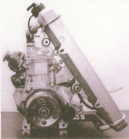
ROTAX FR125 MAX
